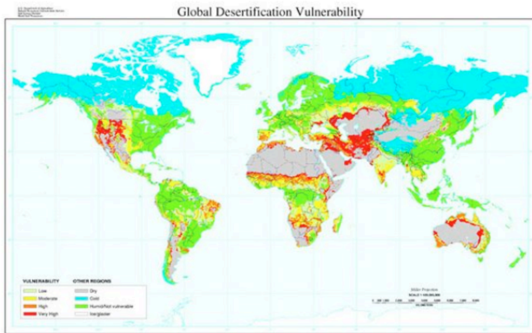
Fig. 2: Global map of desertification vulnerability
