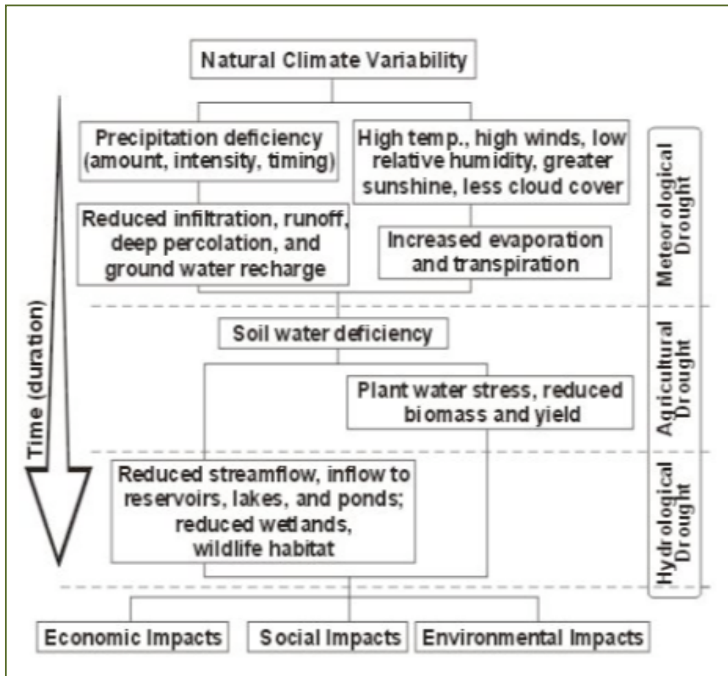
Fig. 1: Climate Impacts and Droughts
